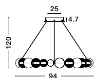
BRILLE • 9695202 Dimmable Gold Aluminium & Acrylic LED 46 Watt 230 Volt 3476Lm 3200K IP20 D: 94 H: 120 cm
