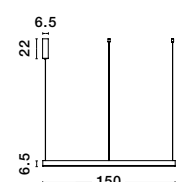
MOTIF . 9530204 Dimmable Sandy Black Aluminium & Acrylic LED 80 Watt 230 Volt 6864Lm 3000K IP20 D: 150 H: 250 cm
