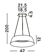
ALBA - 9345655 Dimmable Sandy White Aluminium Outside Champaign Gold Inside LED 40 Watt 230V 1655Lm 3000K IP20 D: 42 H: 200 cm
