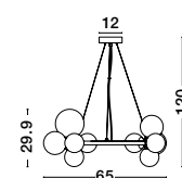
ODILLIA • 9009249 Matt Black Metal & Glass LED G9 11x6 Watt 230 Volt IP20 Bulb Excluded Two ways of mounting D: 65 H: 120 cm
