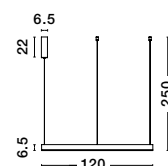
MOTIF . 9530200 Dimmable Sandy White Aluminium & Acrylic LED 70 Watt 230 Volt 5984Lm 3000K IP20 D: 120 H: 250 cm
