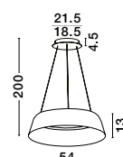
ALBA - 9345657 Dimmable Sandy White Aluminium Outside Champaign Gold Inside LED 50 Watt 230V 2196Lm 3000K IP20 D: 54 H: 200 cm
