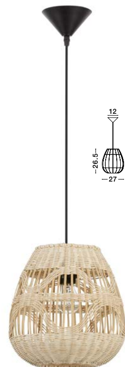
MARLO - 9586500 Natural Rattan Black Fabric Wire & Base LED E27 1x12 Watt 230 Volt IP20 Bulb Excluded D: 27 H 1 : 26.5 H 2 : 180 cm
