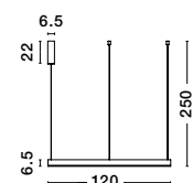
MOTIF . 9530201 Dimmable Sandy White Aluminium & Acrylic LED 70 Watt 230 Volt 5984Lm 3000K IP20 D: 120 H: 250 cm
