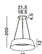
ALBA - 9345656 Dimmable Sandy Black Aluminium Outside Champaign Gold Inside LED 40 Watt 230V 1655Lm 3000K IP20 D: 42 H: 200 cm
