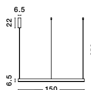
MOTIF . 9530203 Dimmable Sandy White Aluminium & Acrylic LED 80 Watt 230 Volt 6864Lm 3000K IP20 D: 150 H: 250 cm
