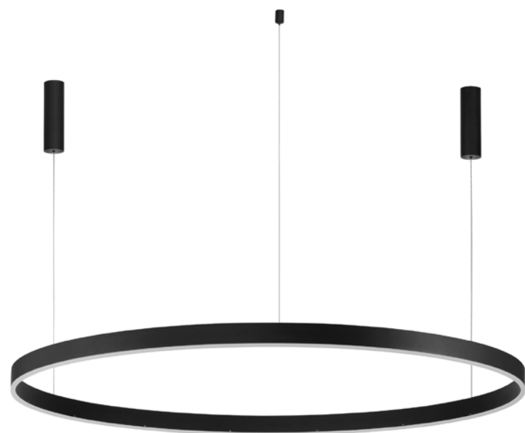
MOTIF . 9530204 Dimmable Sandy Black Aluminium & Acrylic LED 80 Watt 230 Volt 6864Lm 3000K IP20 D: 150 H: 250 cm
