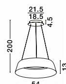
ALBA - 9345658 Dimmable Sandy Black Aluminium Outside Champaign Gold Inside LED 50 Watt 230V 2196Lm 3000K IP20 D: 54 H: 200 cm
